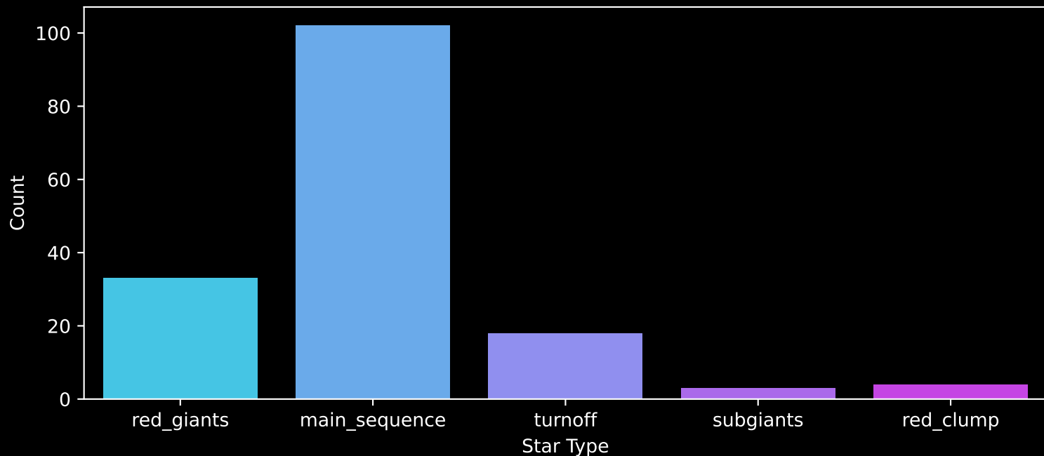
APOGEE DR17 Field: [086+77] Count plot of Star Type
