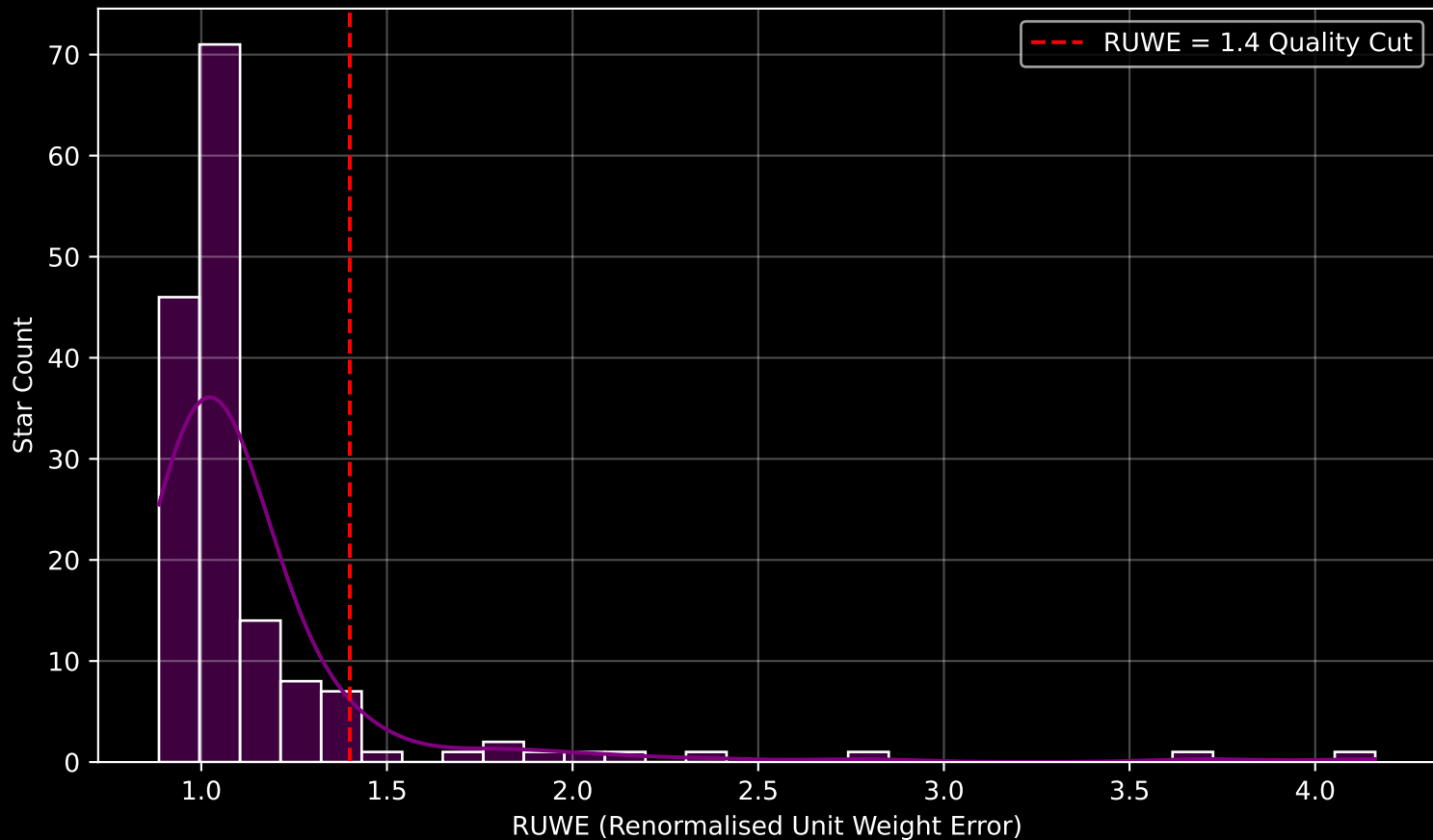
GAPOGEE DR17 Field [086+77] RUWE Distribution (n= 157)
