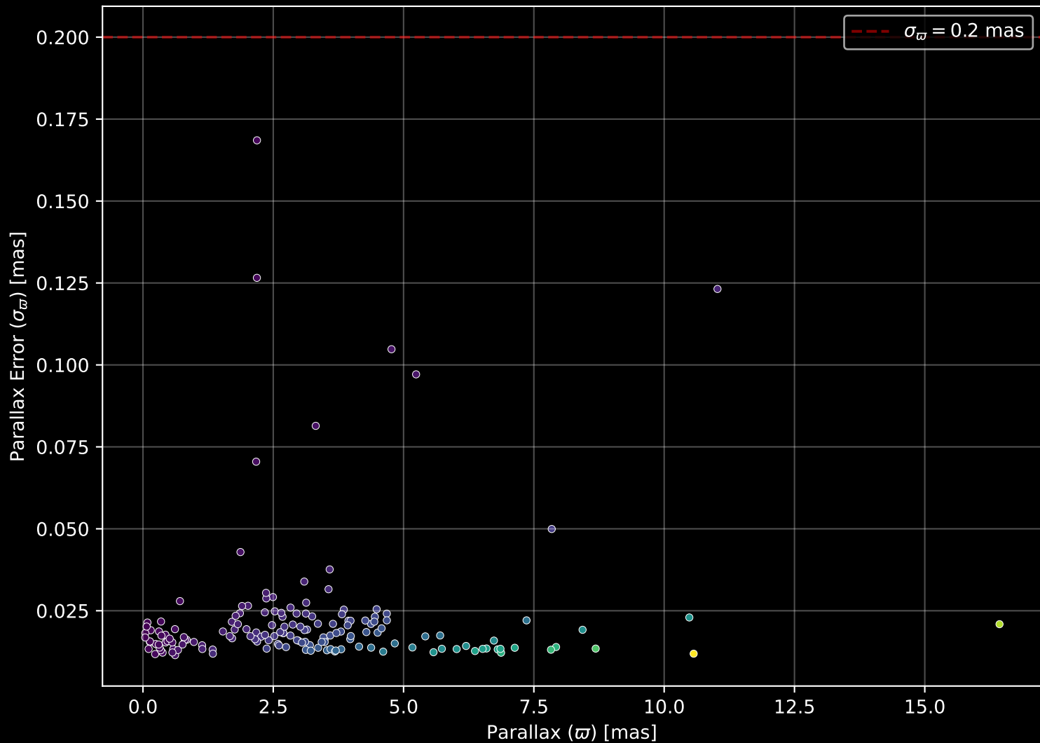
APOGEE DR17 Field: [086+77] Parallax Quality (n= 160)
