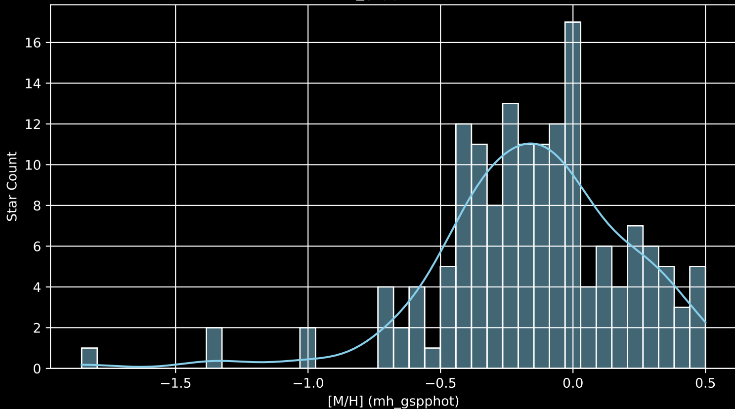
APOGEE DR17 Field: [086+77 [M/H] (mh_gspphot) (n= 156)
