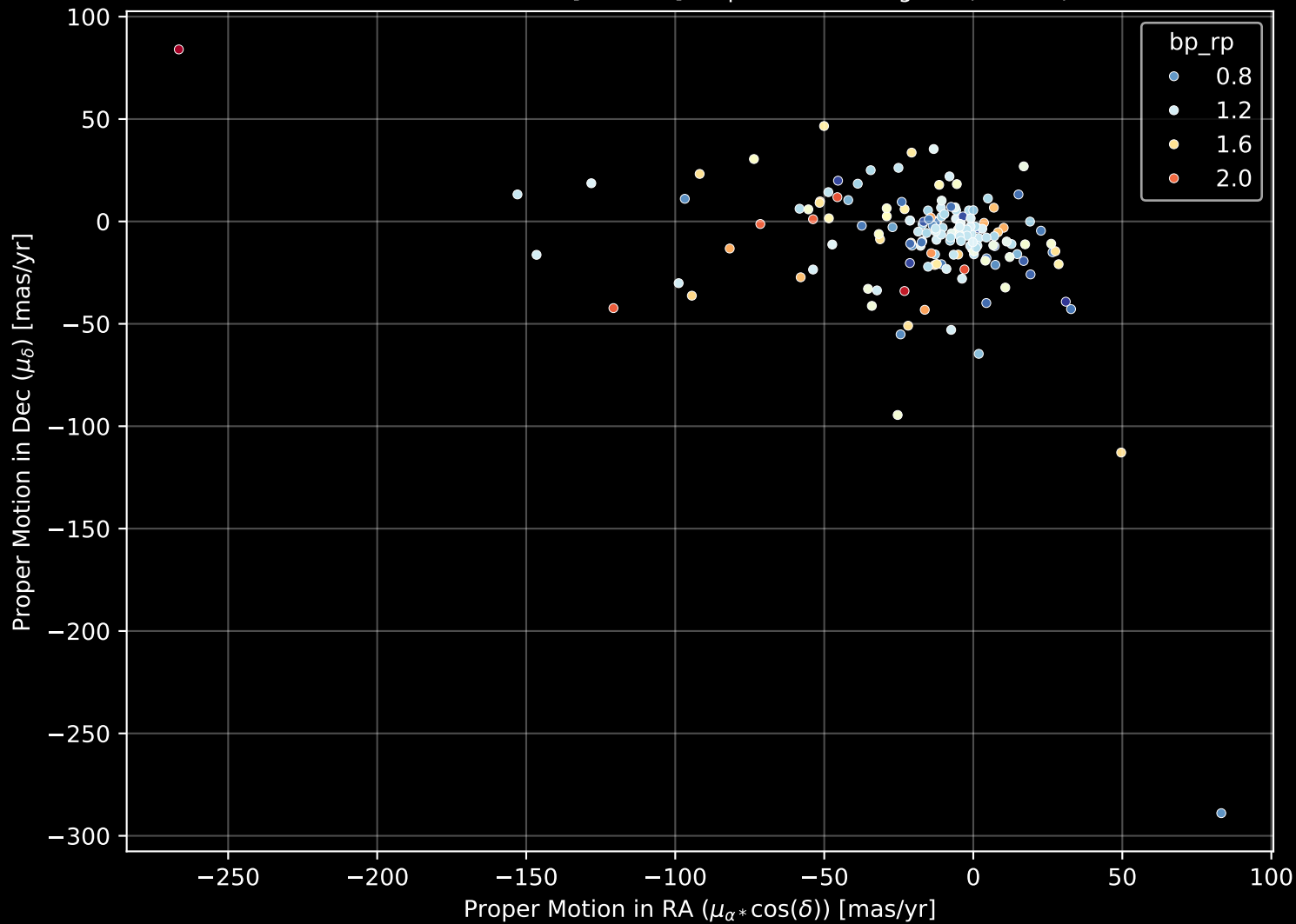
APOGEE DR17 Field: [086+77] Proper Motion Diagram (n= 160)
